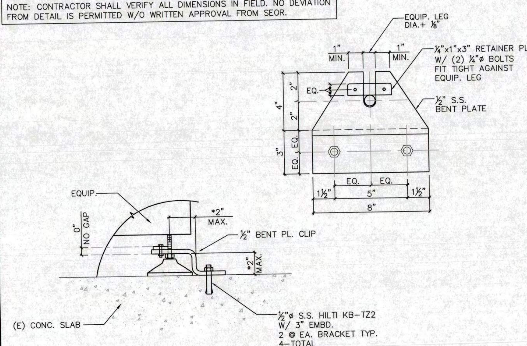
10 ANCHOR DETAILS UNWIND/REWIND
