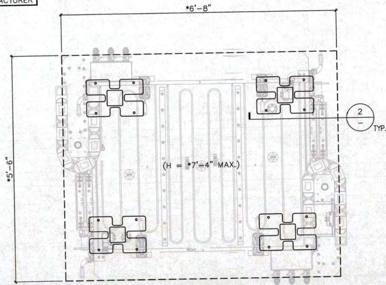
1 ANCHOR LAYOUT FURNACE
