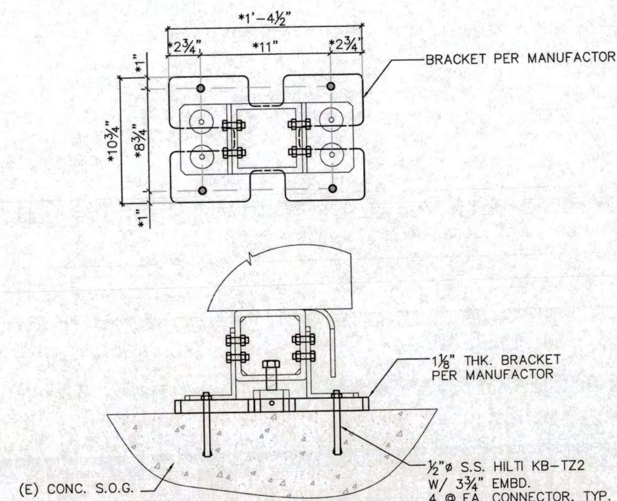
2 ANCHOR DETAILS FURNACE
