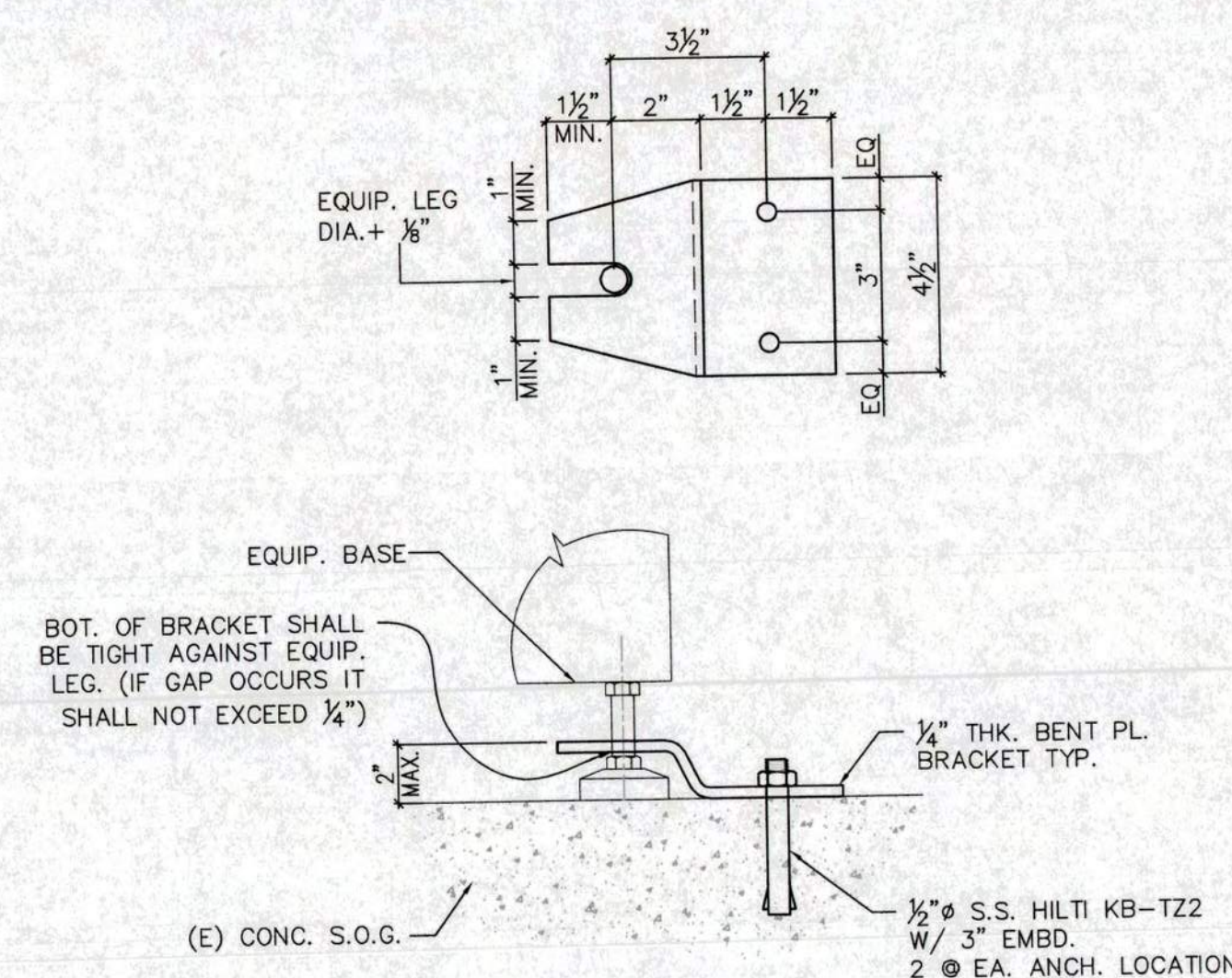
6 ANCHOR DETAILS GAS PANEL
