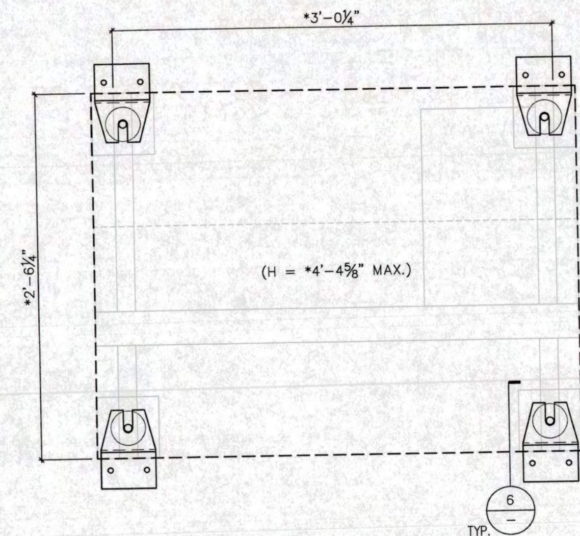
5 ANCHOR LAYOUT GAS PANEL
