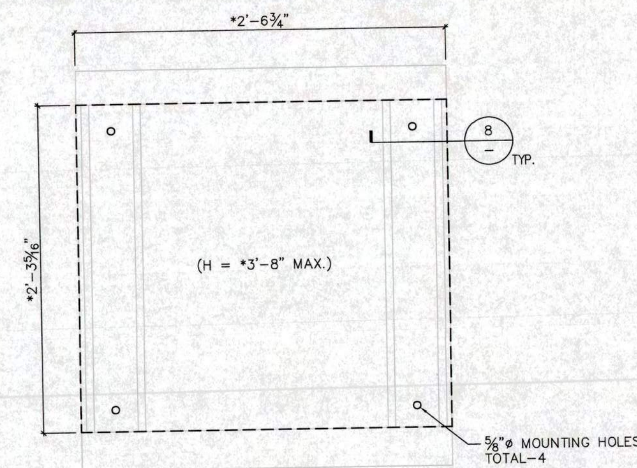
3 ANCHOR LAYOUT ELECTRICAL CABINET
