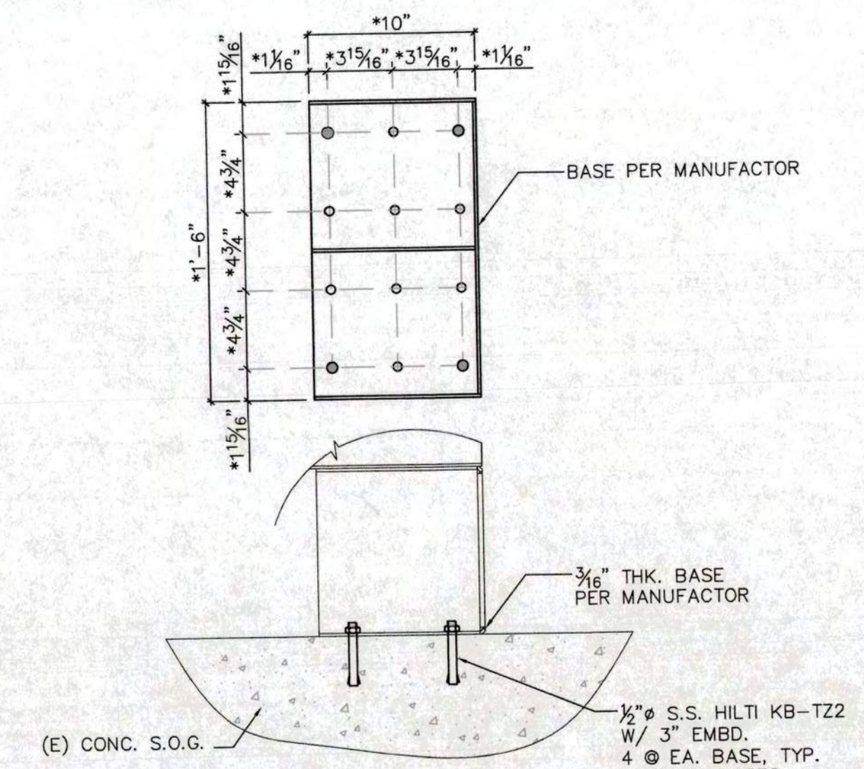
4 ANCHOR DETAILS ELECTRICAL CABINET
