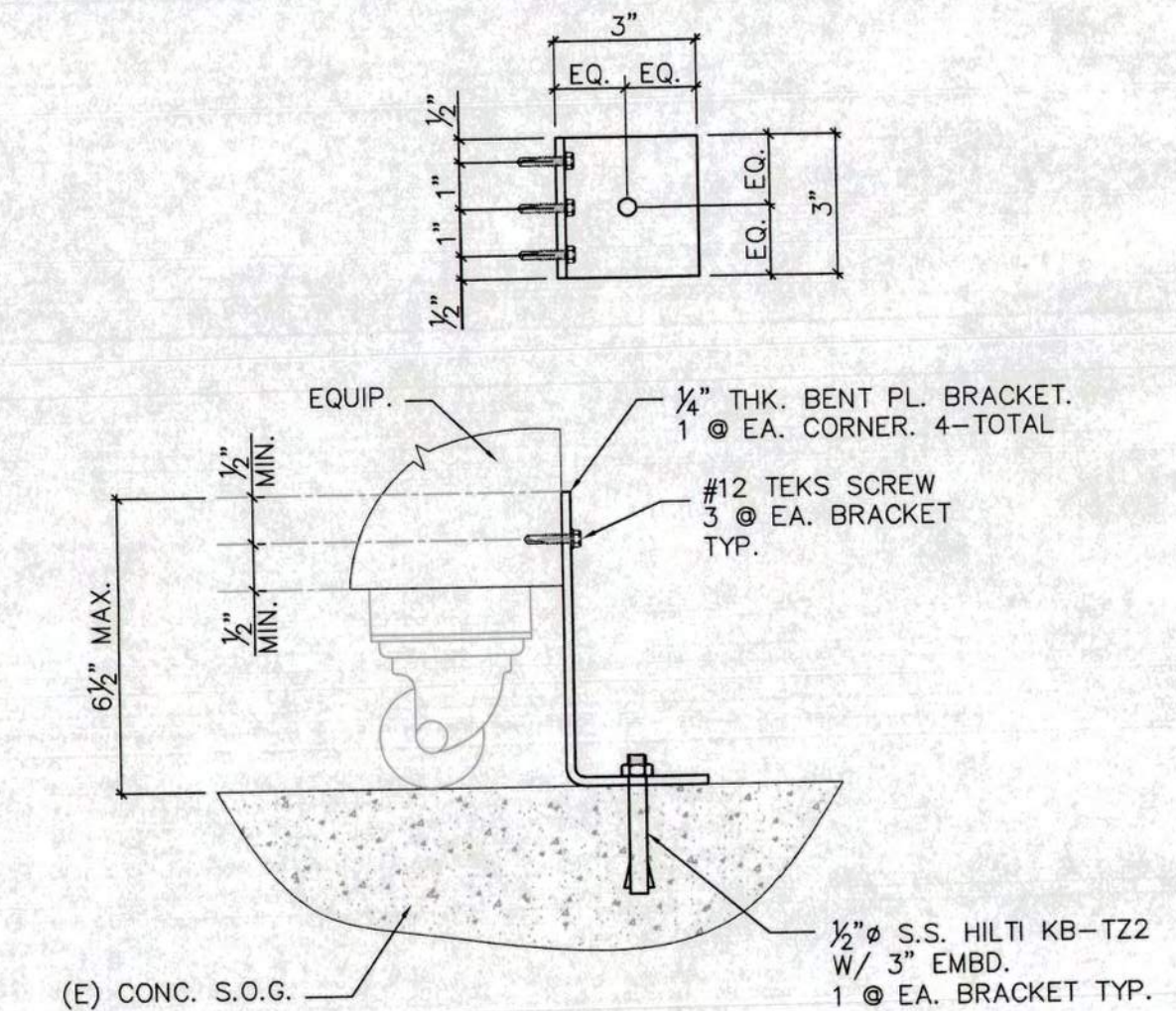
12 ANCHOR DETAILS ESUC UNIT
