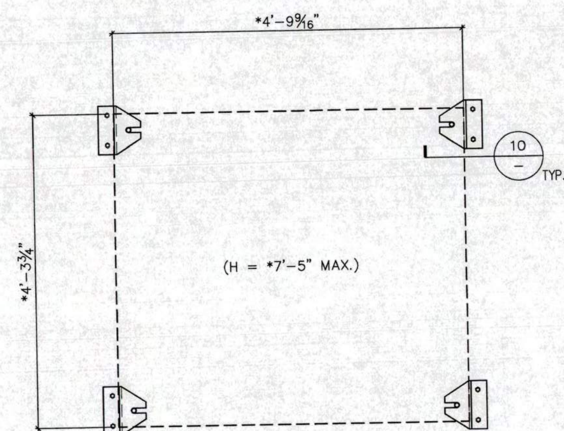
9 ANCHOR LAYOUT UNWIND/REWIND
