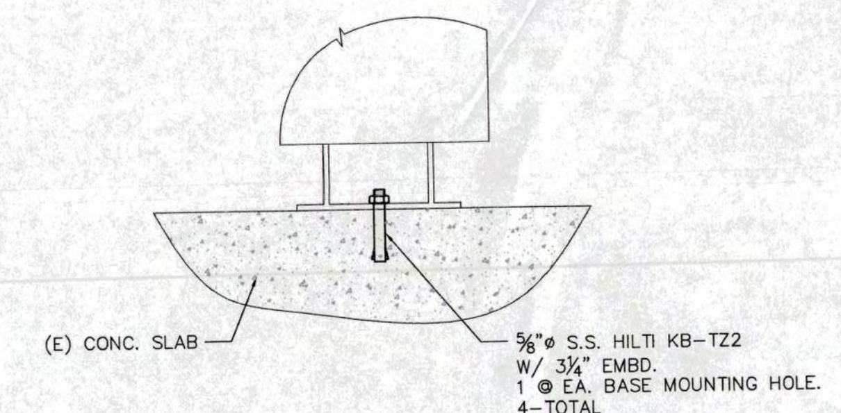
8 ANCHOR DETAIL TRANSFORMER
